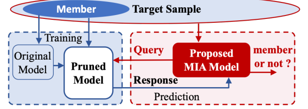
Figure 3: Framework of membership inference attacks (MIA) against neural network pruning.
