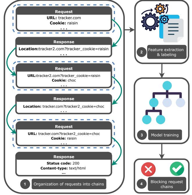
Figure 1: KHALEESI: (1) We first organize network and JavaScript-layer requests into chains. (2) We then label the request chains with ad and tracker blocking filter lists and extract features from them. (3) We use the extracted features to train a machine learning model and (4) use it to detect and block advertising and tracking request chains. The example cookie syncing request chain in (1) demonstrates the benefit of sequential context leveraged by KHALEESI. Specifically, the dotted blue blocks represent the context utilized by existing approaches in isolation. Whereas the green arrows represent the increasing sequential context utilized by KHALEESI.
