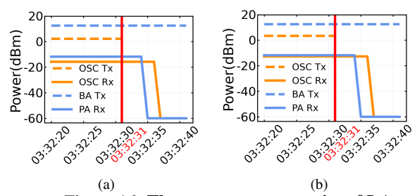
Figure 16: The power outage at site of LA.
