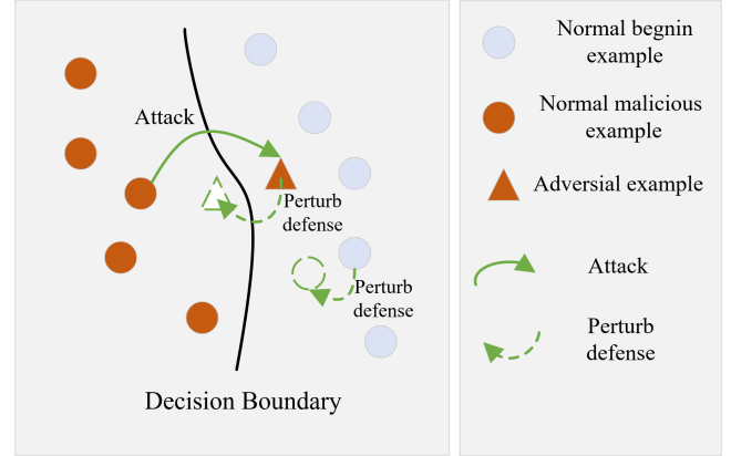
Figure 4: Attack and Defense of Android Malware
