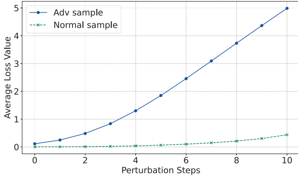
Figure 6: Loss Comparison: Adversarial Samples vs. Normal Samples with Increasing Perturbation Steps
