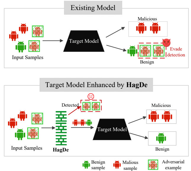
Figure 1: How HagDe Enhances AMD Target Model
