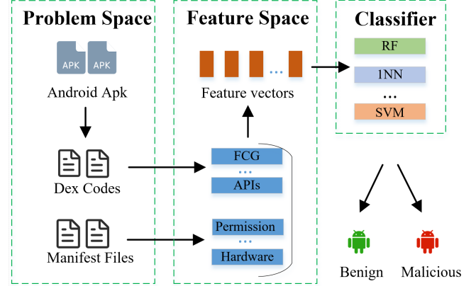
Figure 2: Learning-based Android Malware Detection
